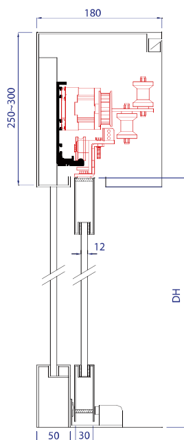
Cross section
