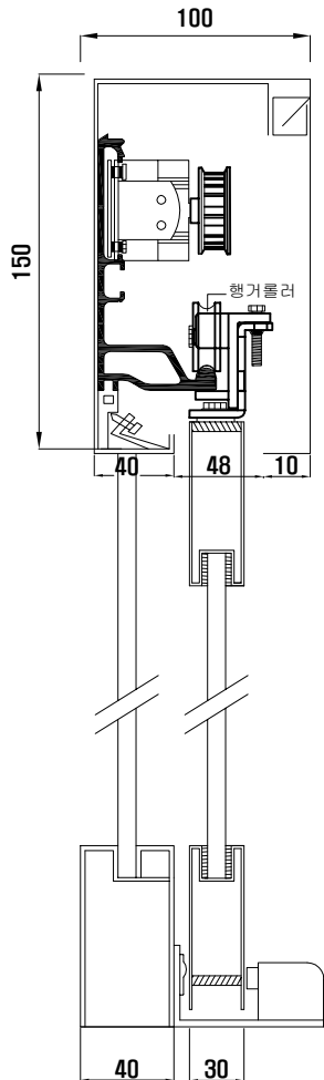
VERTICAL SECTION
